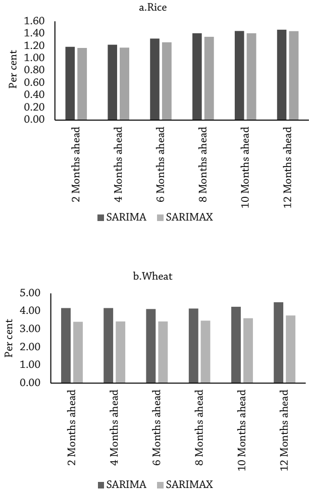
Figure 4.20 Rolling Window (60 Months) Forecast Comparison for Rice and Wheat based on RMSE (per cent)
