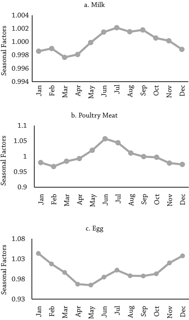
Figure 3.5 Seasonality in CPI Livestock and Poultry (Based on Seasonal Factors over the Last 10 Years)
